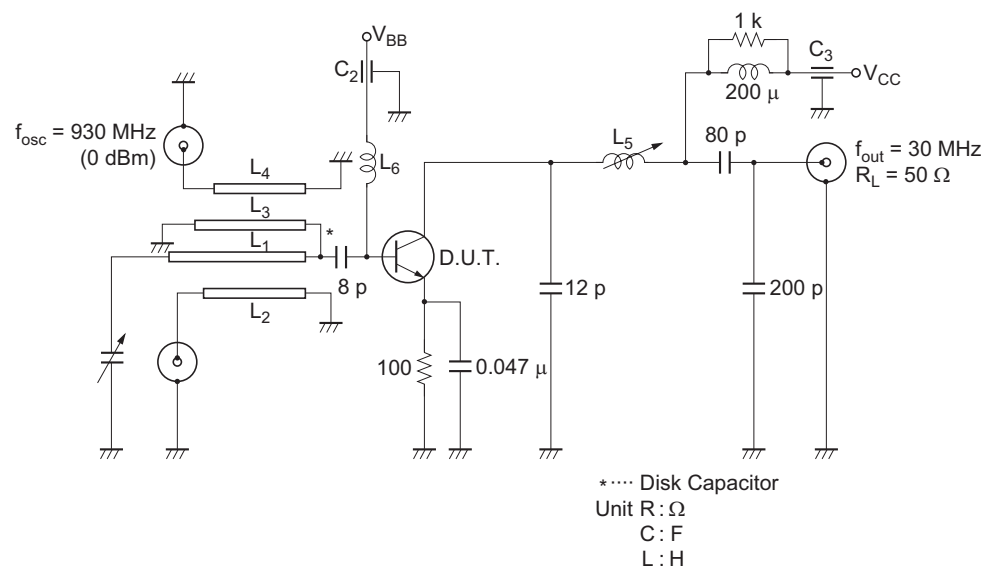
Conversion Gain, Noise Figure Test Curcuit
