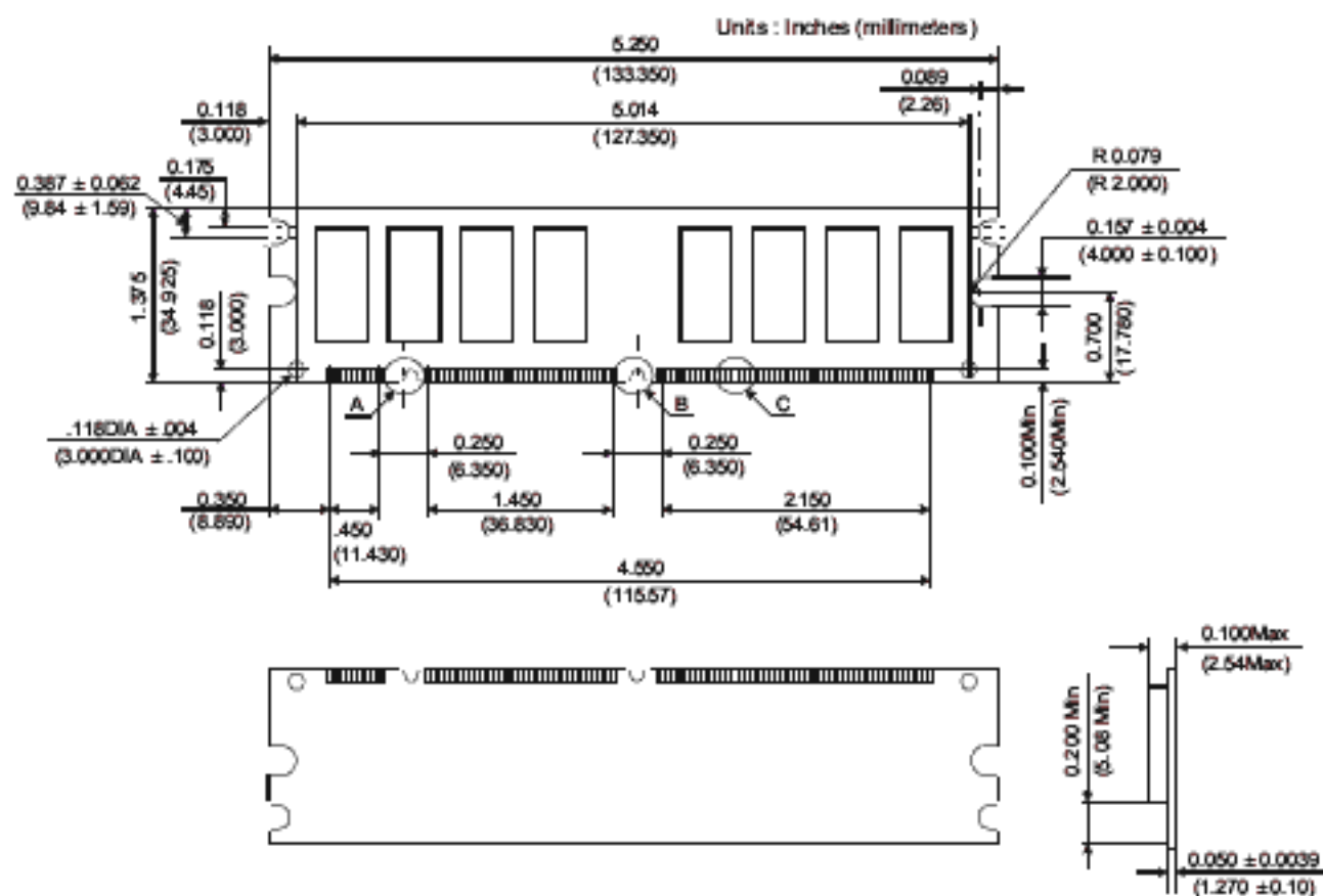
Figure 1: KVR133X64C3/64 168-Pin SDRAM Module
