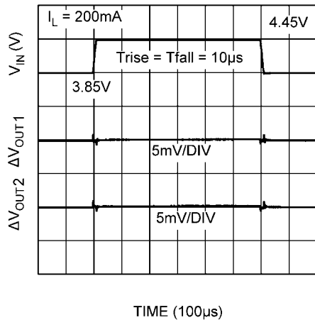
Line Transient, 200mA per Channel
