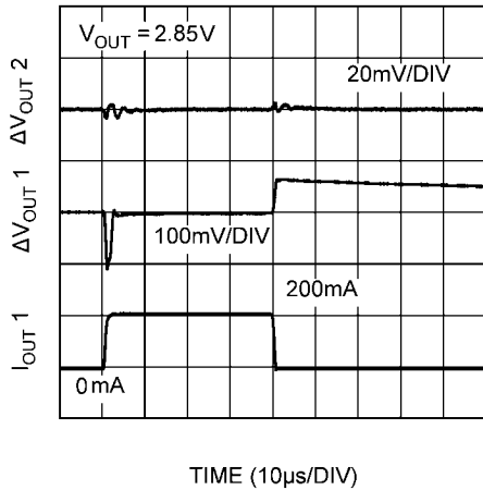
Vout 1 Load Transient 0 to 200mA
