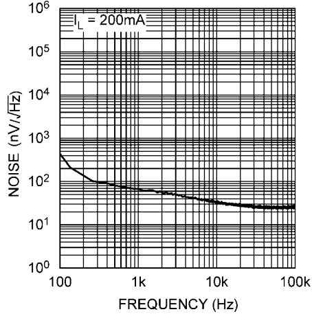
Noise Density
