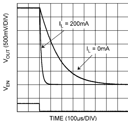
Shutdown Characteristics
