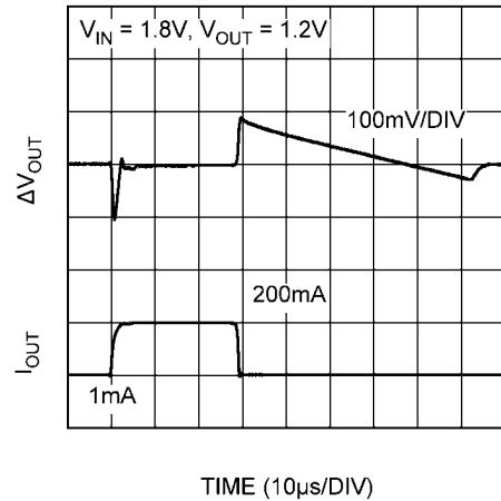
Load Transient. V_{IN} = 1.8V , V_{OUT} = 1.2V
