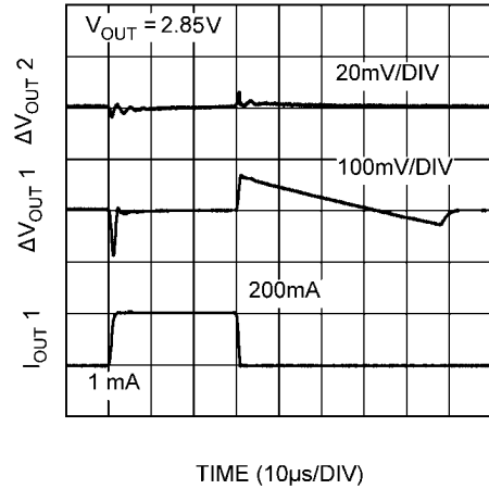
Vout 1 Load Transient 1 to 200mA
