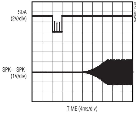
HEADPHONE STARTUP WAVEFORM
