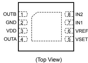
Terminal Diagram
