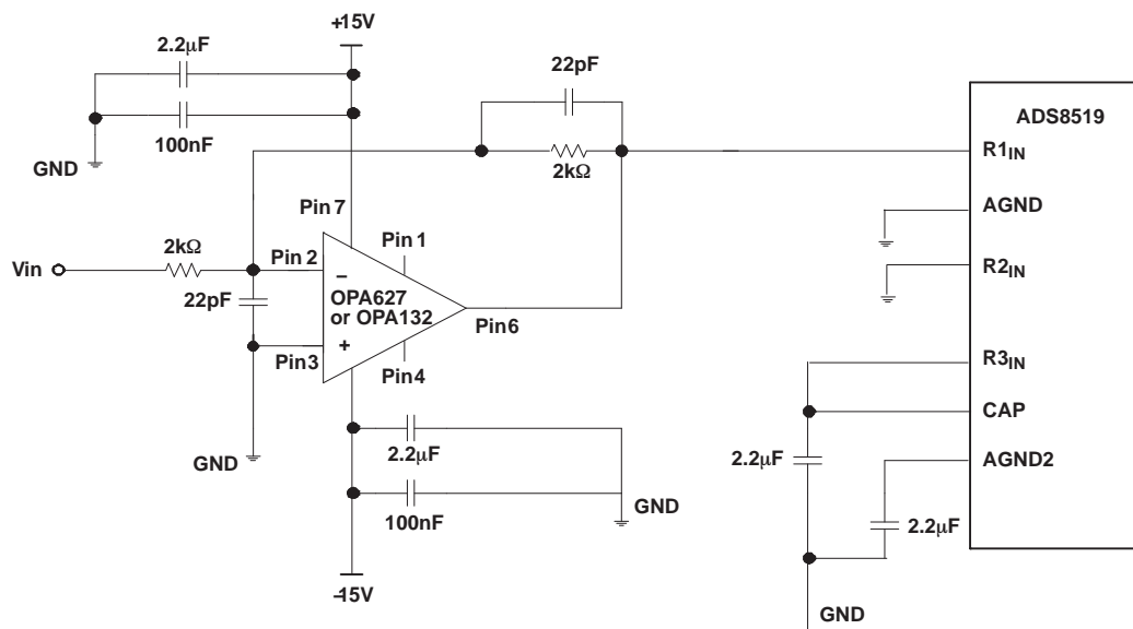
Figure 31. Typical Driving Circuitry ( \pm 10 V, No Trim)
