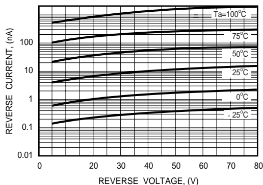
FIG. 4 - REVERSE CHARACTERISTICS
