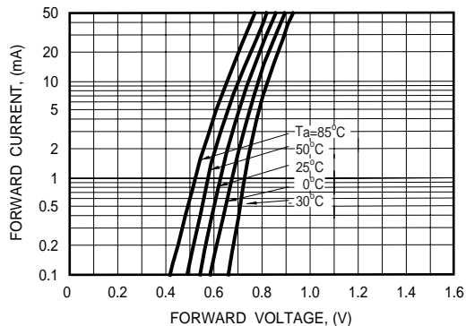
FIG. 2 - FORWARD CHARACTERISTICS
