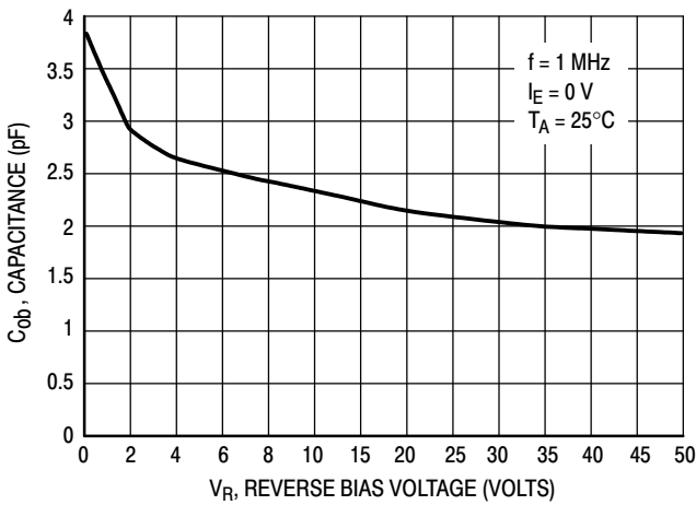
Figure 34. Output Capacitance
