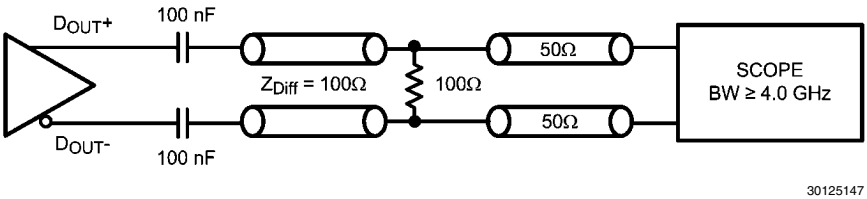
FIGURE 5. Serializer CML Output Load and Transition Times
