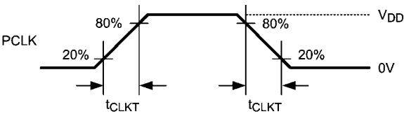
FIGURE 8. Serializer Input Clock Transition Times
