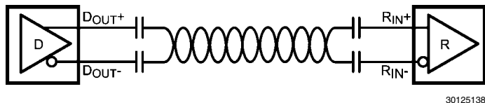
FIGURE 30. AC-Coupled Application
