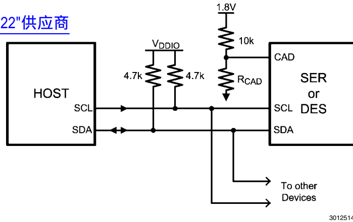
FIGURE 24. Serial Control Bus Connection
