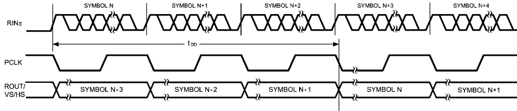
FIGURE 14. Deserializer Delay
