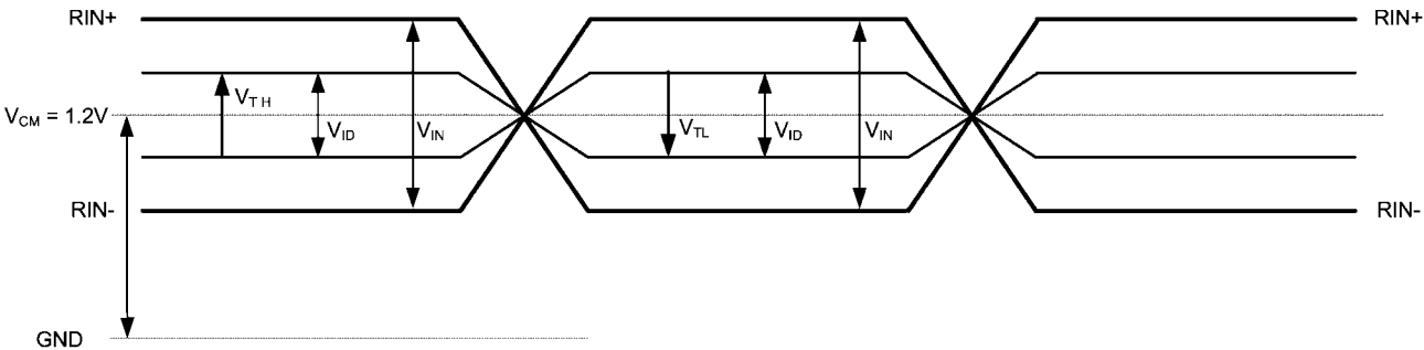
FIGURE 7. Low-Voltage Differential VTH/VTL Definition Diagram
