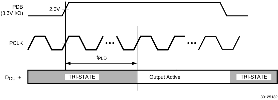
FIGURE 10. Serializer Data Lock Time
