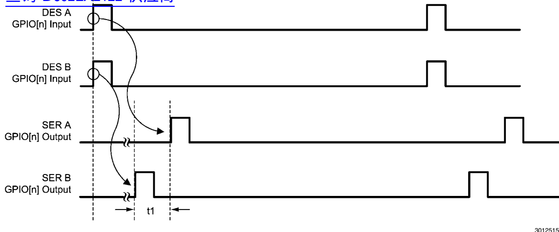
FIGURE 25. GPIO Delta Latency
