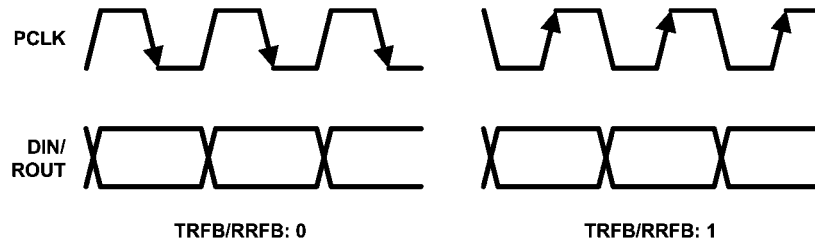
FIGURE 29. Programmable PCLK Strobe Select
