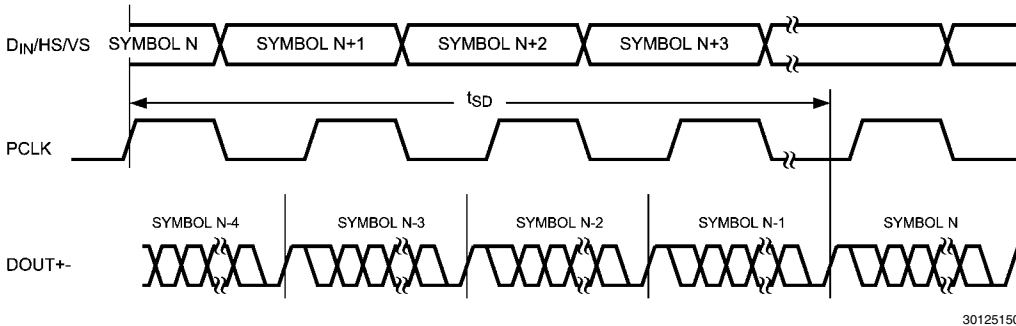
FIGURE 11. Serializer Delay
