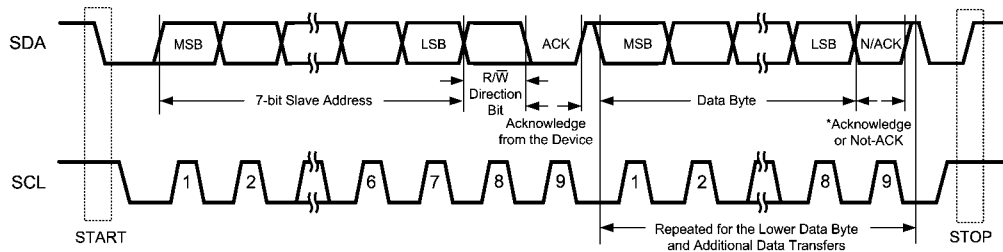
FIGURE 22. Basic Operation
