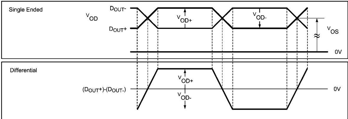
FIGURE 6. Serializer VOD DC Diagram
