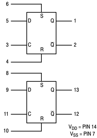
BLOCK DIAGRAM
