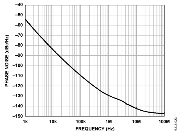
Figure 23. Internal VCO Phase Noise (Absolute), Direct-to-LVPECL @ 2050 MHz
