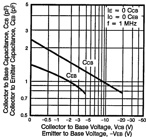
DEVICE CAPACITANCE
