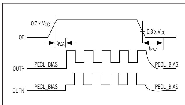
Figure 3. LVPECL Output Timing Diagram When OE Is Enabled and Disabled
