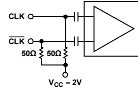
Figure 30. Typical AC-Coupled or DC-Coupled PECL Configuration (See Table 8 for LVPECL DC-Coupling Limitations)
