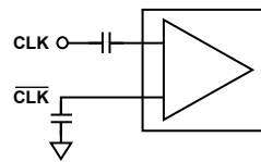
Figure 31. Typical 1.8 V CMOS Configurations for Short Trace Lengths (See Table 8 for CMOS Compatibility)
