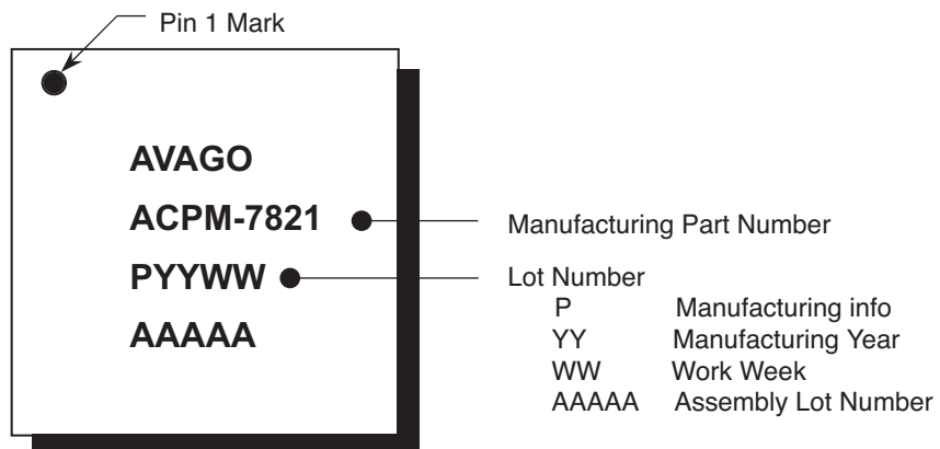
Figure 9. Marking Specifications.
