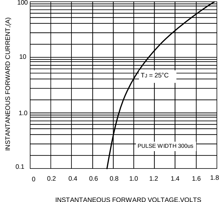
FIG.4-TYPICAL FORWARD CHARACTERISTICS
