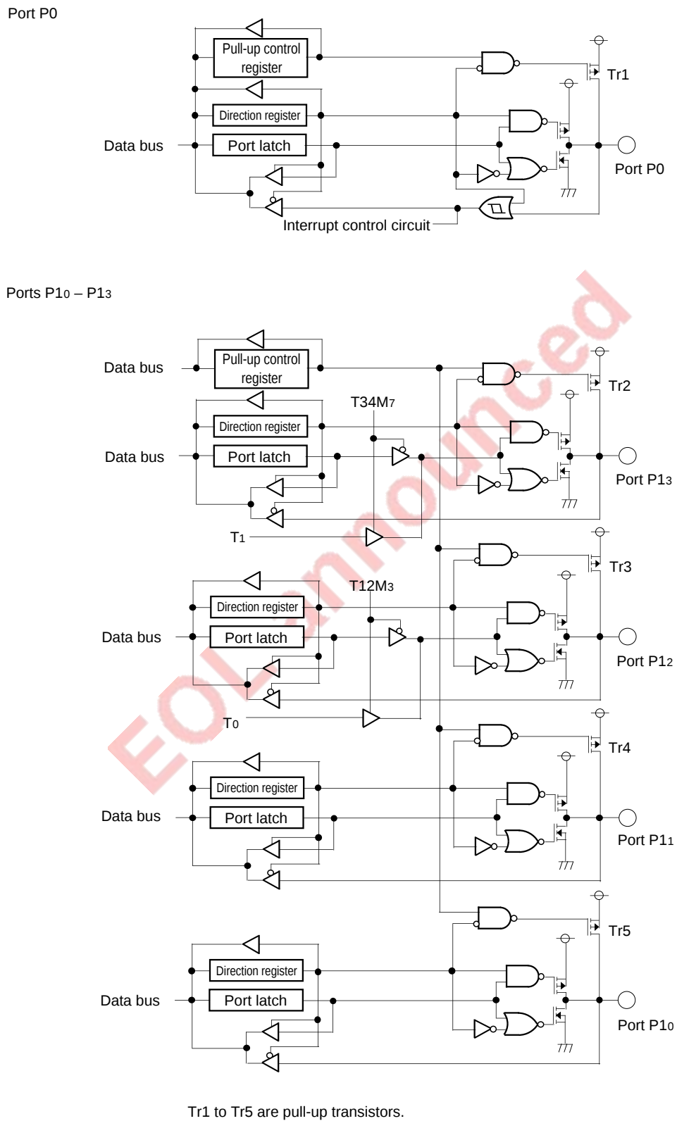
Fig. 19 Block diagram of ports P0, P10–P13
