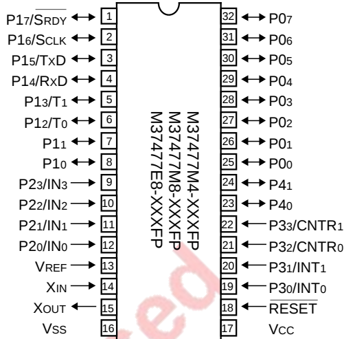
Outline 32P2W-A (Note 2)
