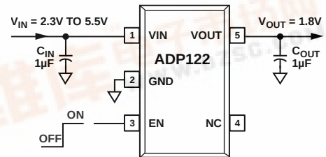
Figure 1. ADP122 with Fixed Output Voltage
