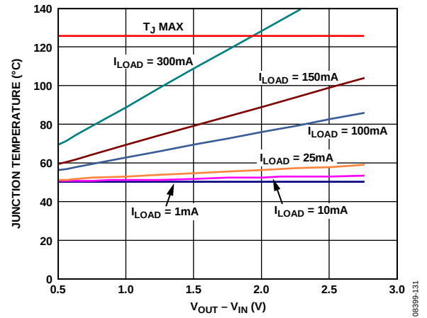
Figure 37. Junction Temperature vs. Power Dissipation, 500 mm 2 of PCB Copper, T_A = 50^\circ\text{C}
