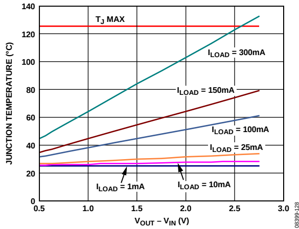
Figure 34. Junction Temperature vs. Power Dissipation, 500 mm 2 of PCB Copper, T_A = 25^\circ\text{C}
