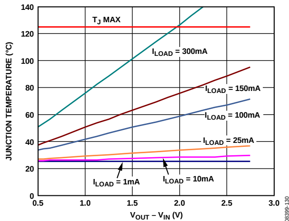
Figure 36. Junction Temperature vs. Power Dissipation, 0 mm 2 of PCB Copper, T_A = 25^\circ\text{C}
