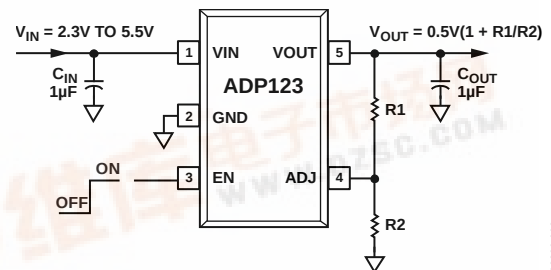
Figure 2. ADP123 with Adjustable Output Voltage
