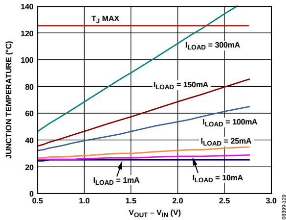
Figure 35. Junction Temperature vs. Power Dissipation, 100 mm 2 of PCB Copper, T_A = 25^\circ\text{C}
