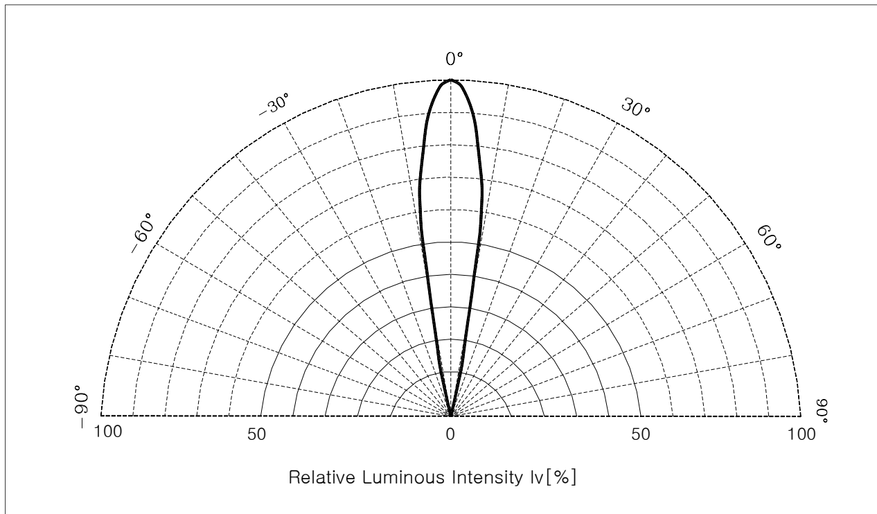
Fig. 5 Radiation Diagram
