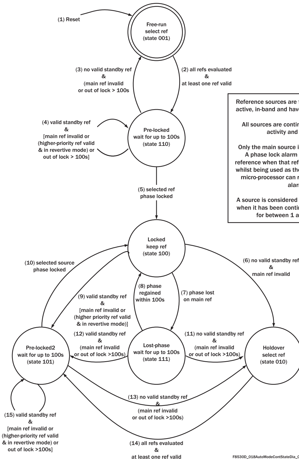
Figure 4 Automatic Mode Control State Diagram
