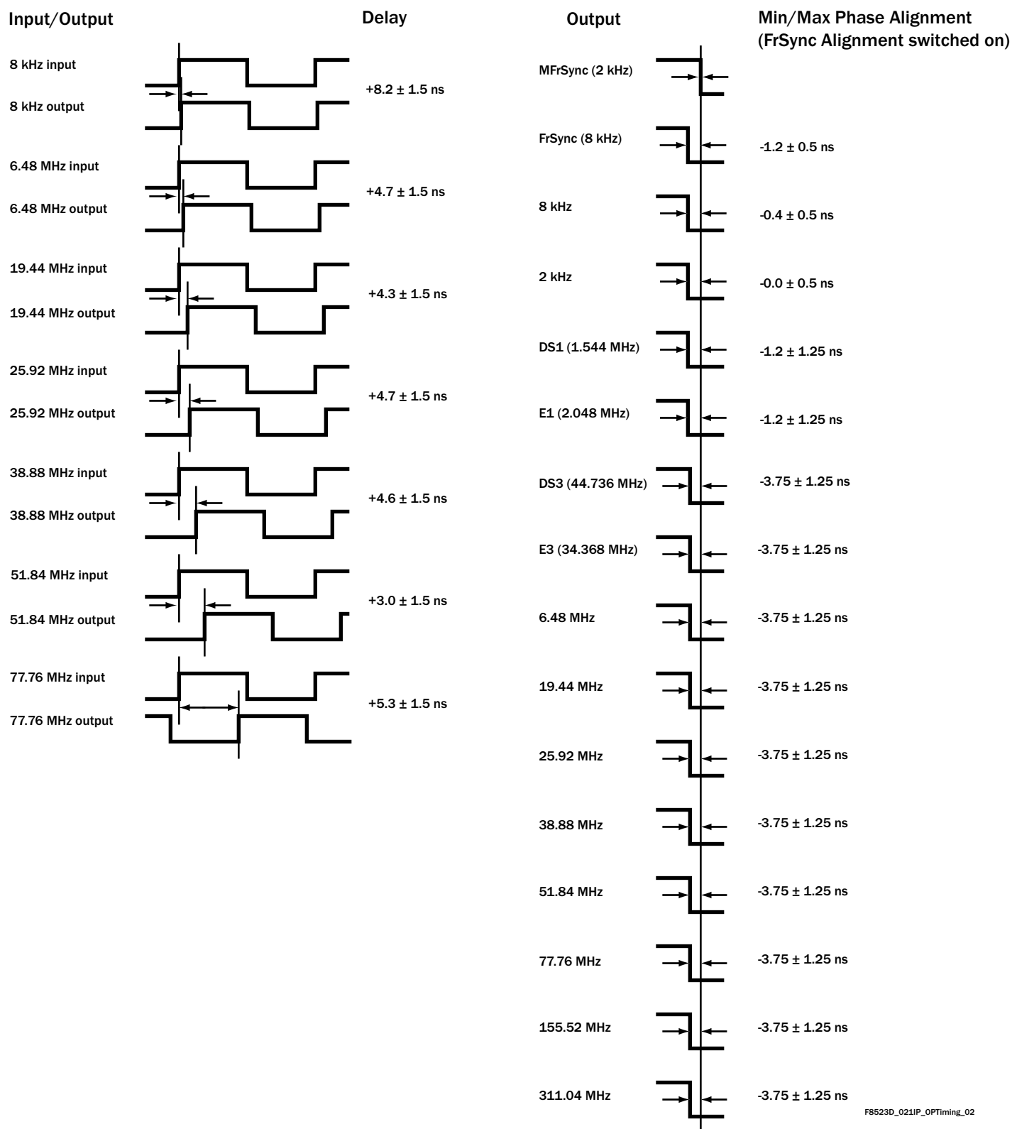
Figure 17 Input/Output Timing with Phase Build-out Off
