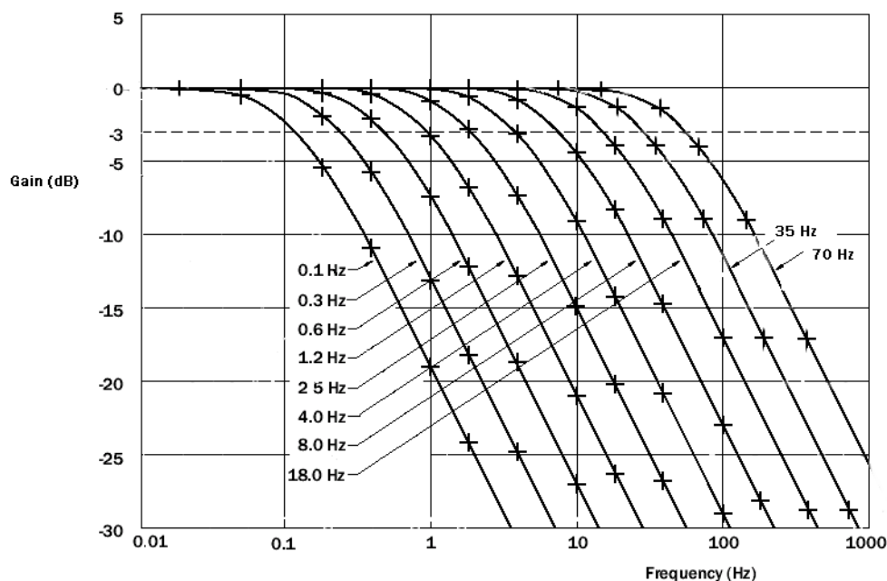
Figure 7 Sample of Wander and Jitter Measured Transfer Characteristics
