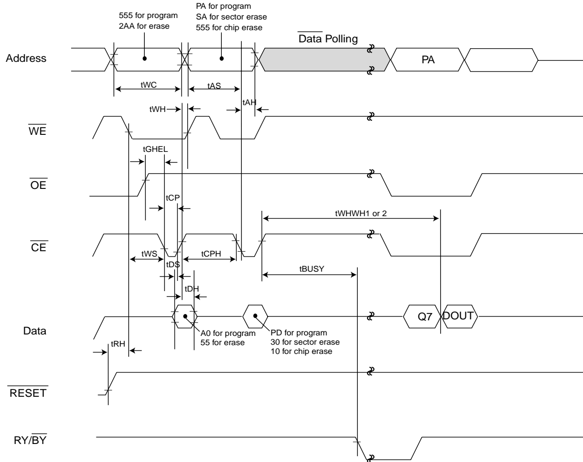
Fig 10. \overline{CE} CONTROLLED PROGRAM TIMING WAVEFORM
