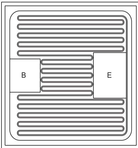
BACKSIDE COLLECTOR
