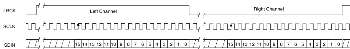
Figure 32. Right-Justified Serial Audio Formats
