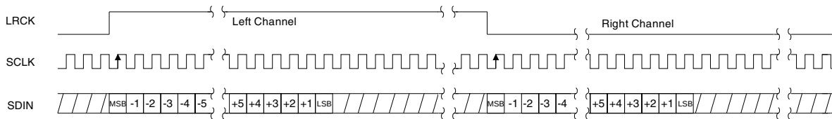
Figure 31. Left-Justified Serial Audio Formats
