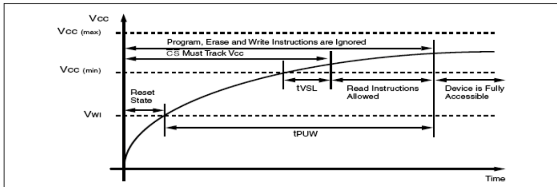
Figure 22. Power-up Timing
