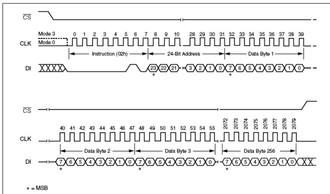
Figure 12. Page Program Instruction Sequence Diagram
