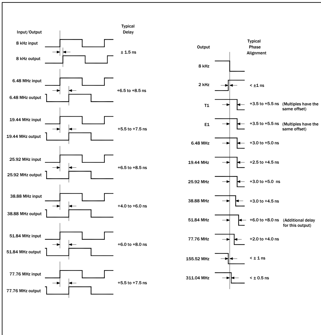
Figure 18. Input/Output Timing
