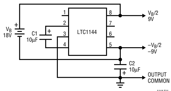
Figure 11. Battery Splitter
