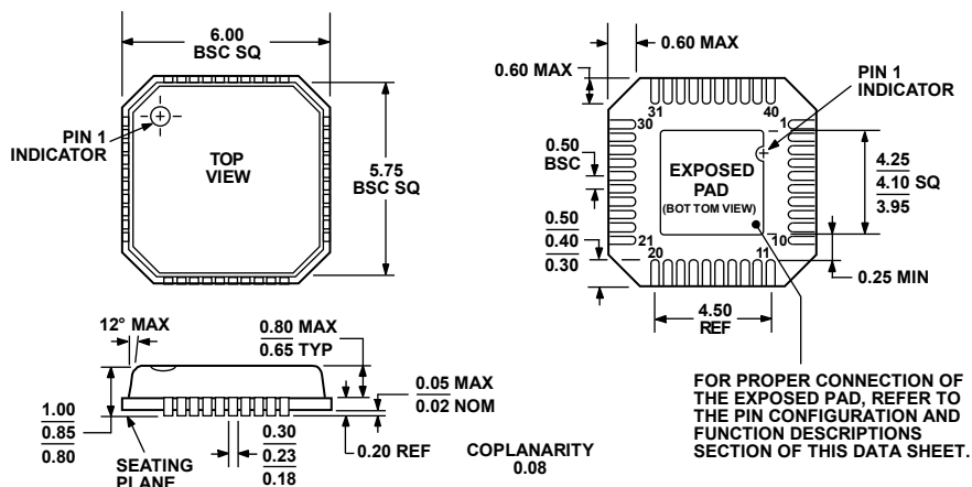
Figure 79. 40-Lead Lead Frame Chip Scale Package [LFCSP_VQ]
