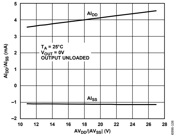
Figure 8. A_{1DD}/A_{1SS} vs. AV_{1DD}/AV_{1SS}
