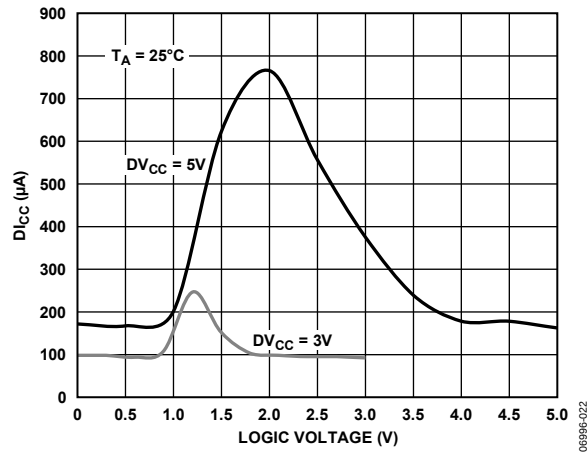
Figure 7. D_{1CC} vs. Logic Input Voltage
