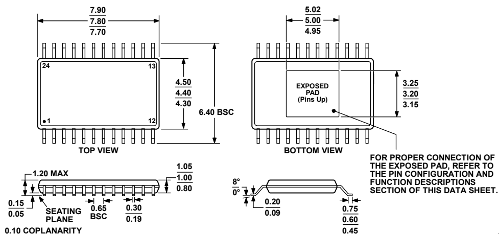
Figure 78. 24-Lead Thin Shrink Small Outline Package, Exposed Pad [TSSOP_EP]
