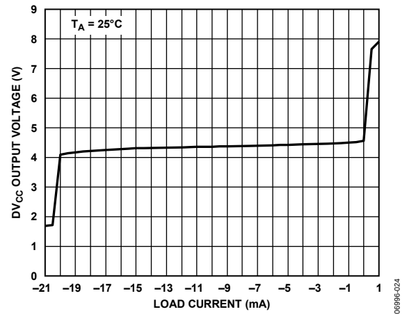
Figure 10. DV_{1CC} Output Voltage vs. Load Current
