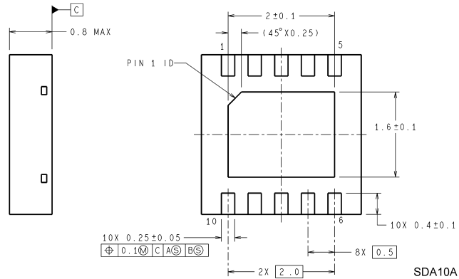
SDA10A: 10-Pin Non-Pullback Leadless Leadframe Package 3.0mm x 3.0mm x 0.8mm
