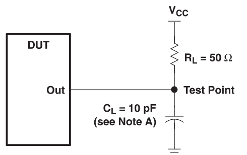
LOAD CIRCUIT HIGH-TO-LOW SLEW-RATE MEASUREMENT
