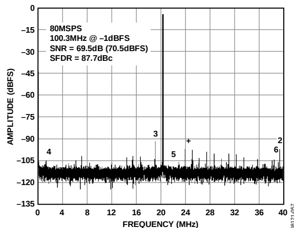
Figure 9. AD9231-80 Single-Tone FFT with f_{IN} = 100.3 MHz
