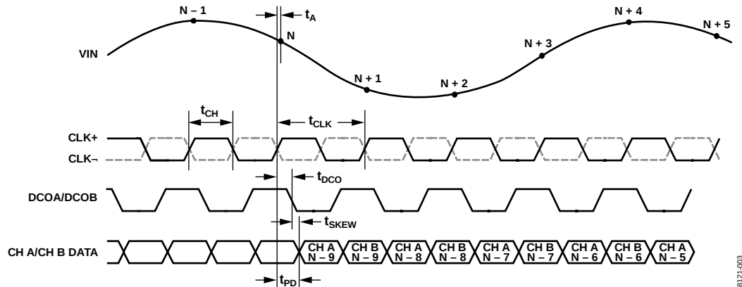
Figure 3. CMOS Interleaved Output Timing
