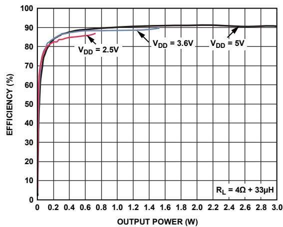
Figure 20. Efficiency vs. Output Power into R_L = 4\Omega + 33\mu H
