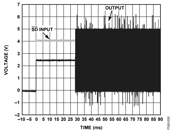
Figure 30. Turn-On Response
