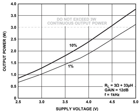
Figure 16. Maximum Output Power vs. Supply Voltage, R_L = 3\Omega + 33\mu H , Gain = 12 dB
