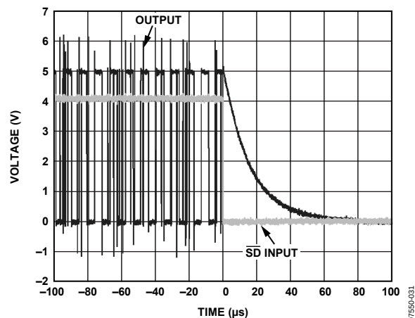
Figure 31. Turn-Off Response
