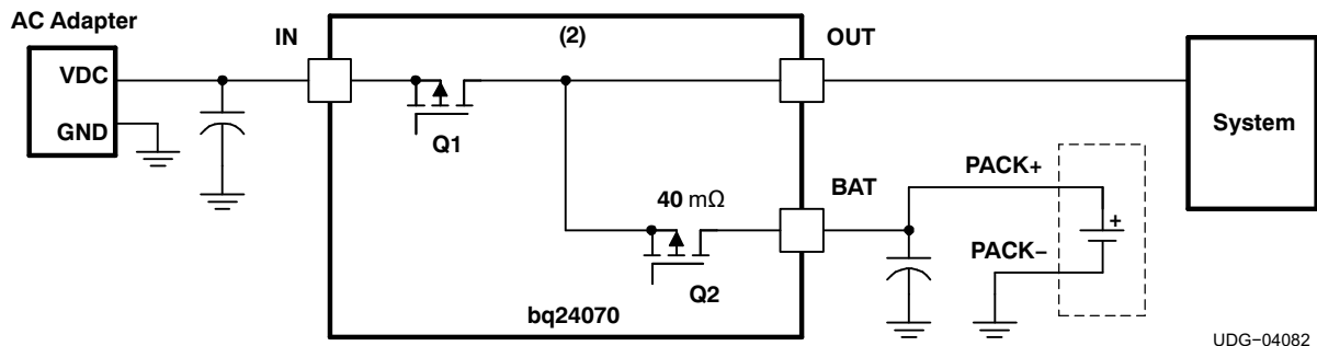
Figure 4. Power-Path Management
