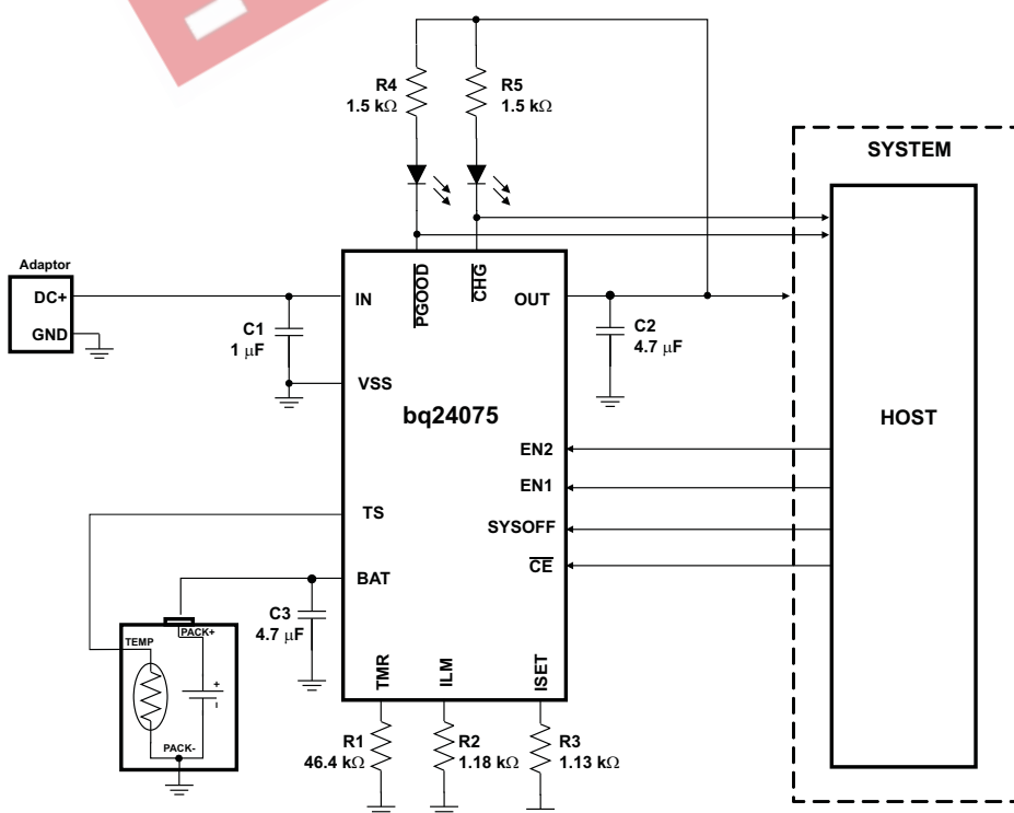
Figure 28. Using bq24075 to Disconnect the Battery from the System
