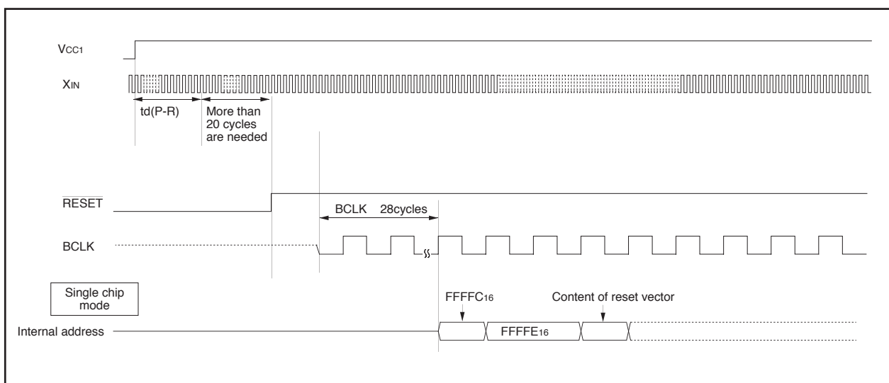
Figure 1.5.2. Reset Sequence
