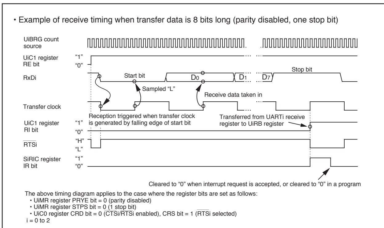
Figure 1.15.2. Receive Operation
