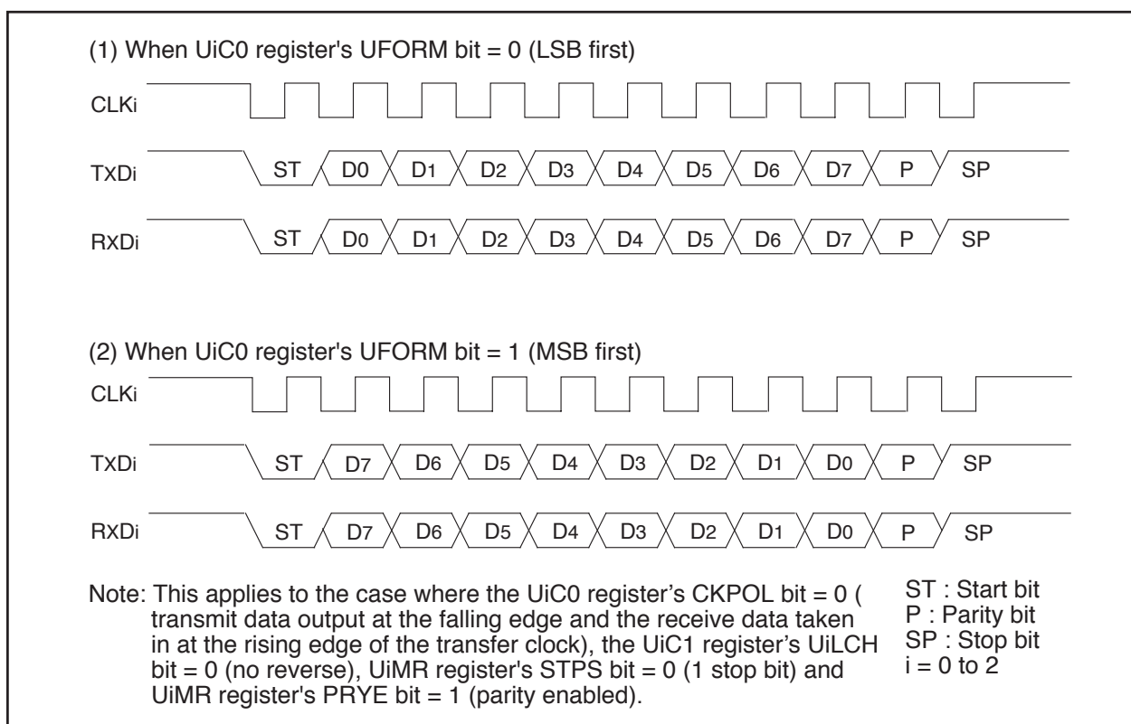
Figure 1.15.3. Transfer Format
