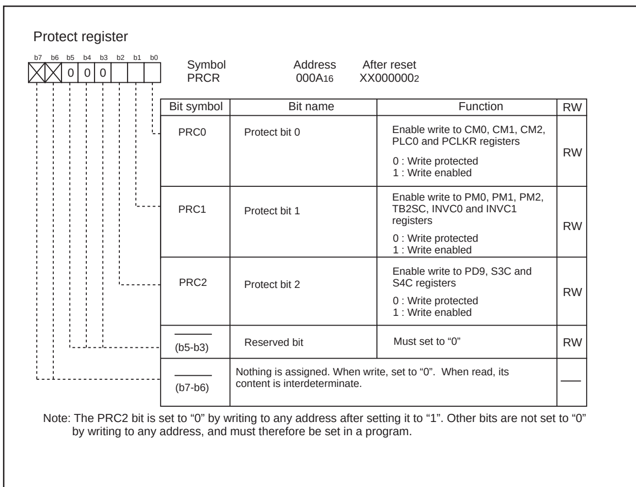
Figure 1.8.1. PRCR Register
