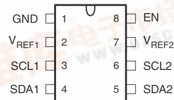
DCU PACKAGE (TOP VIEW)
