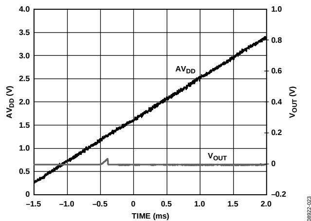
Figure 23. AV_{DD} and V_{OUT} vs. Time on Power-Up
