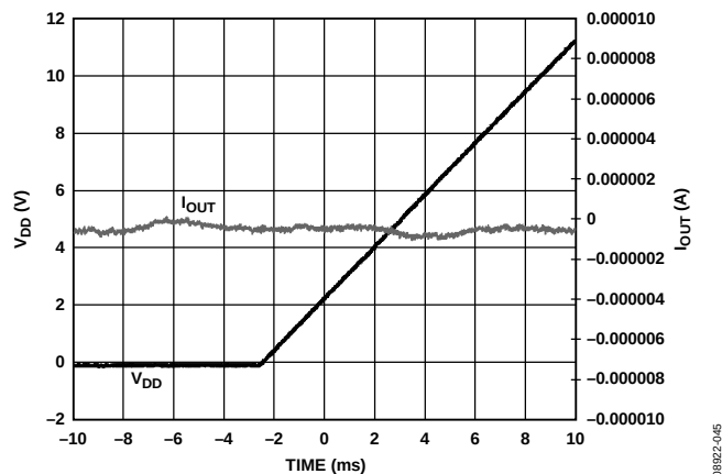
Figure 43. Output Current vs. Time on Power-Up
