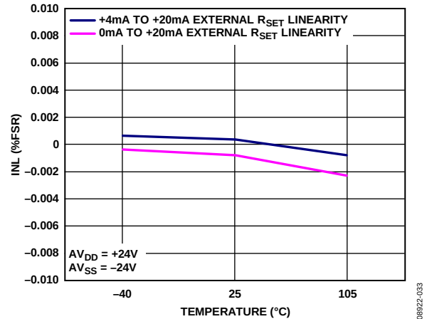
Figure 33. INL vs. Temperature, External R_{SET} Sense Resistor
