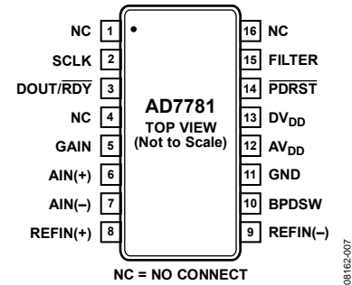
Figure 7. TSSOP Pin Configuration
