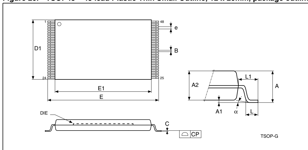
Figure 20. TSOP48 – 48 lead Plastic Thin Small Outline, 12 x 20mm, package outline
