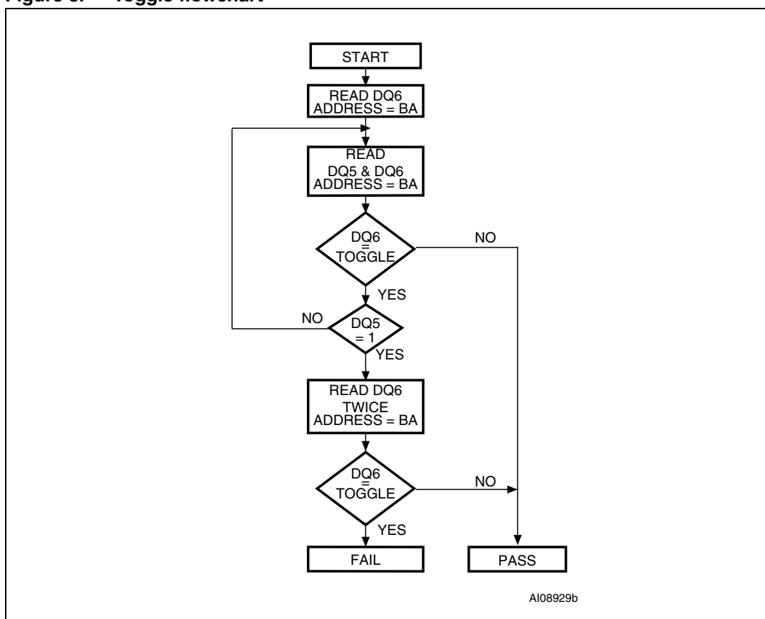
Figure 8. Toggle flowchart
