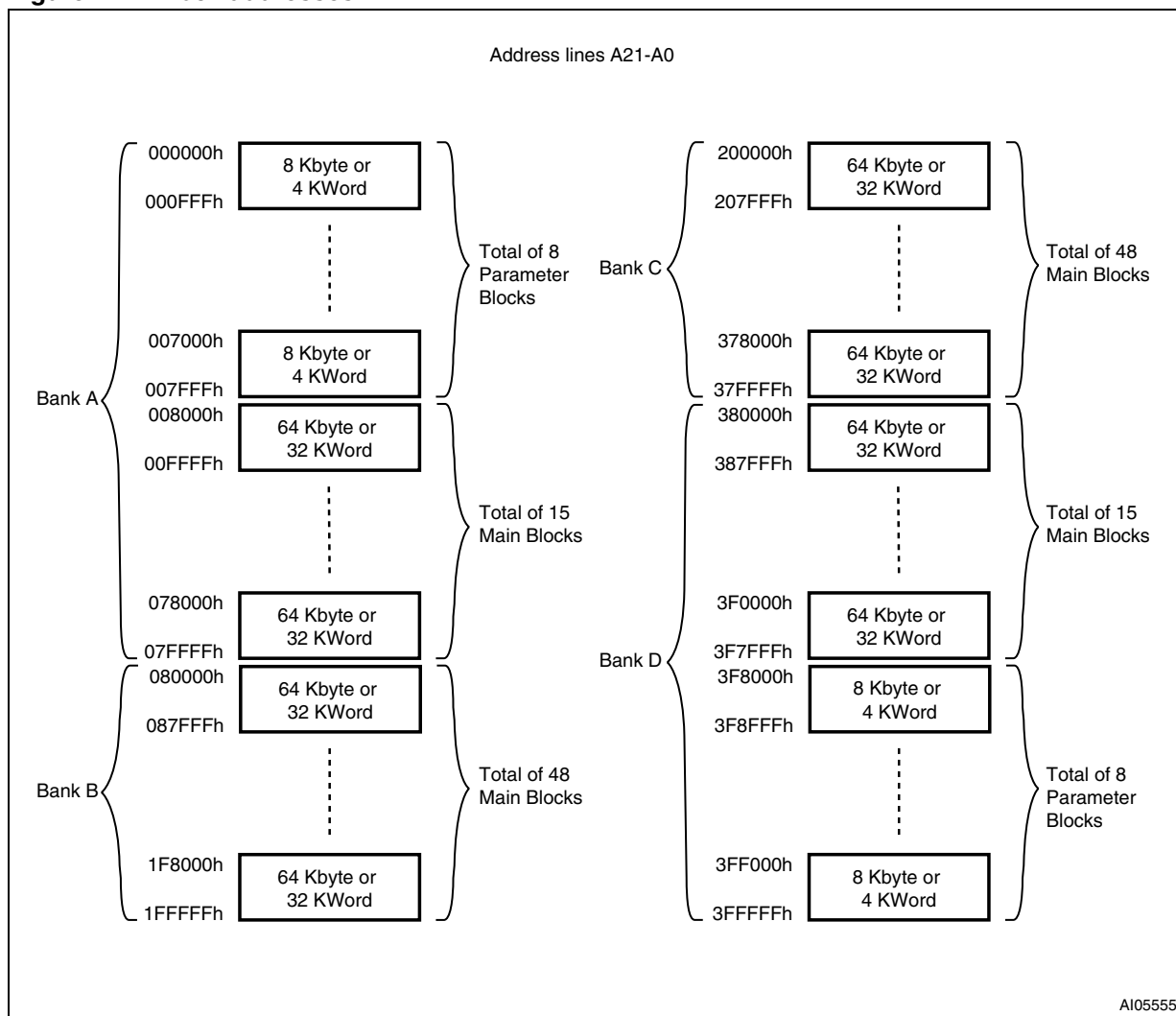
Figure 4. Block addresses
