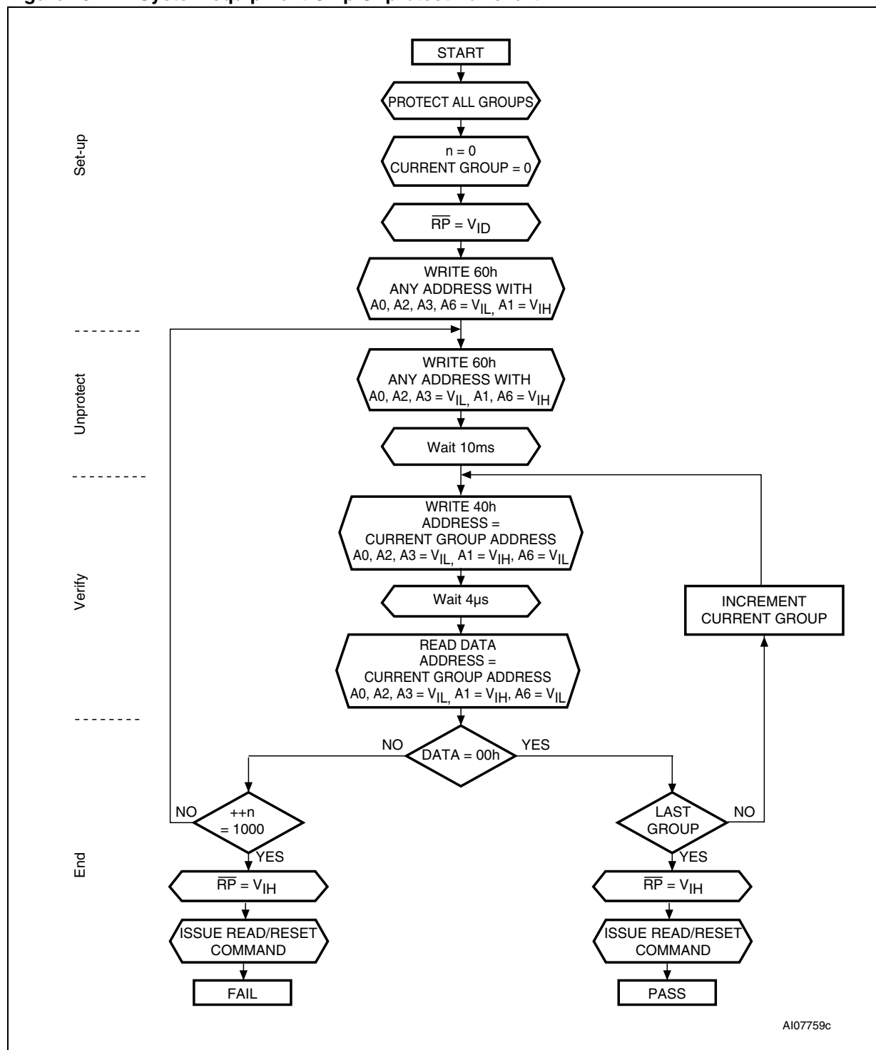
Figure 25. In-System equipment Chip Unprotect flowchart
