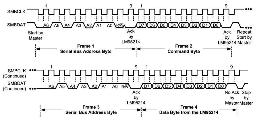
FIGURE 8. SMBus Timing Diagrams
