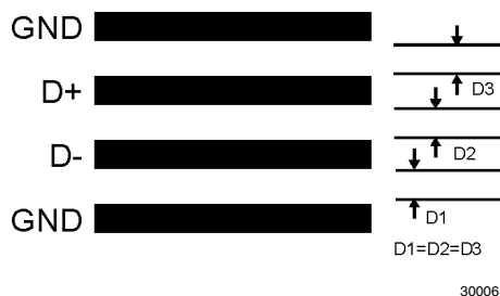
FIGURE 10. Ideal Diode Trace Layout
