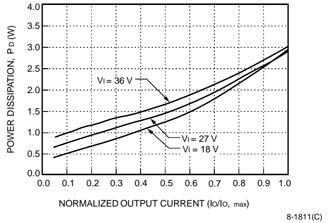
Figure 50. LC010A, B, C Typical Power Dissipation vs. Normalized Output Current at Tc = 25 °C
