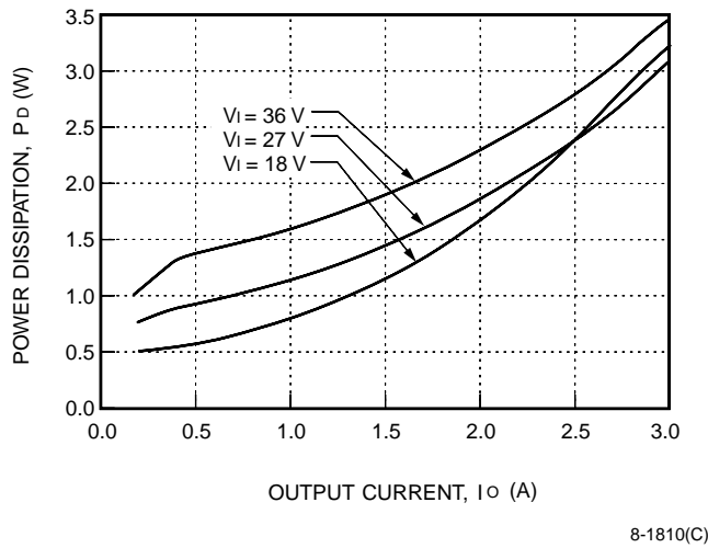
Figure 51. LC010F Typical Power Dissipation vs. Output Current at Tc = 25 °C
