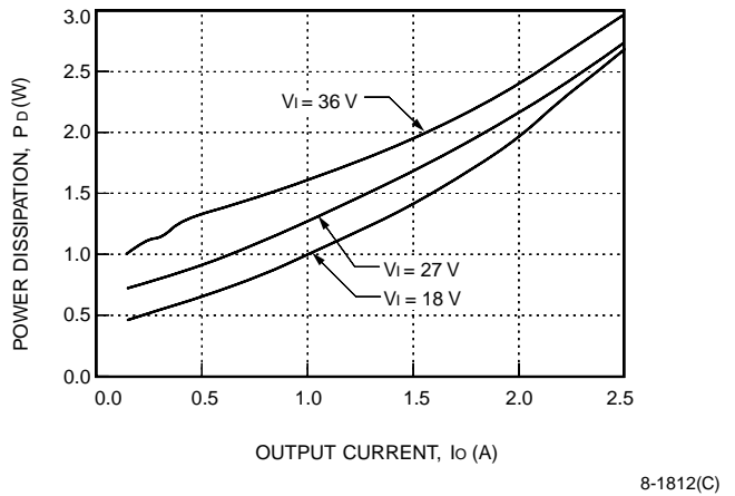
Figure 51. LC010F Typical Power Dissipation vs. Output Current at Tc = 25 °C
