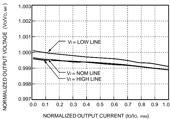
Figure 5. Lx010x/Lx015x Single-Output Load Regulation, Normalized Output Voltage vs. Normalized Output Current at T_c = 25\text{ }^\circ\text{C}
