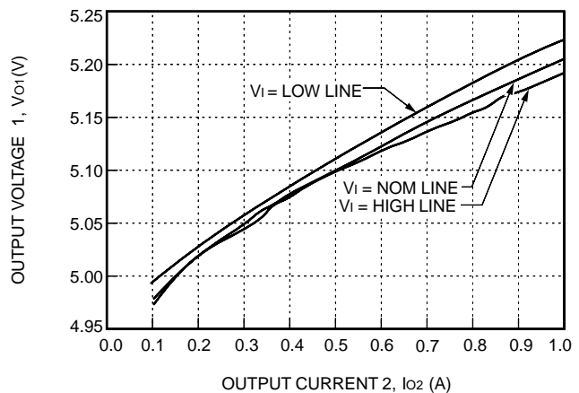
Figure 6. Lx010AJ Typical Load Regulation of Output1 with Fixed I_{o2} = 0.5\text{ A} at T_c = 25\text{ }^\circ\text{C}
