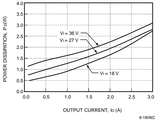
Figure 48. LC010D, 015D Typical Power Dissipation vs. Output Current at Tc = 25 °C
