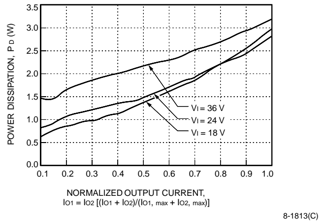
Figure 52. LC010AJ, BK, CL Typical Power Dissipation vs. Normalized Output Current at Tc = 25 °C
