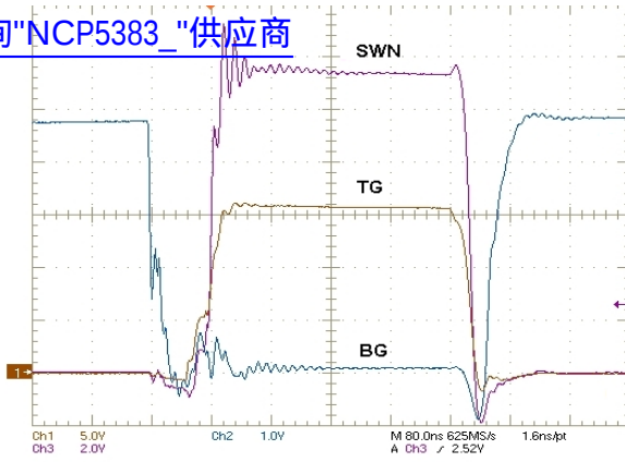
Figure 12. 20 A Sustaining Load
