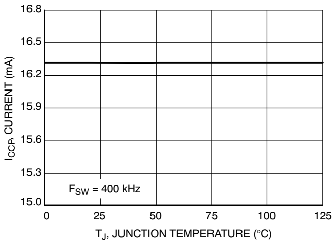
Figure 8. I_{CCP} Current vs. Temperature
