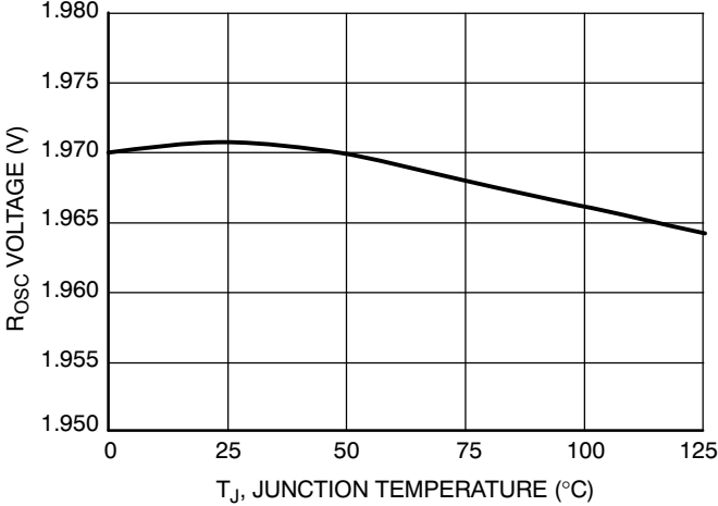
Figure 10. R osc Voltage vs. Temperature
