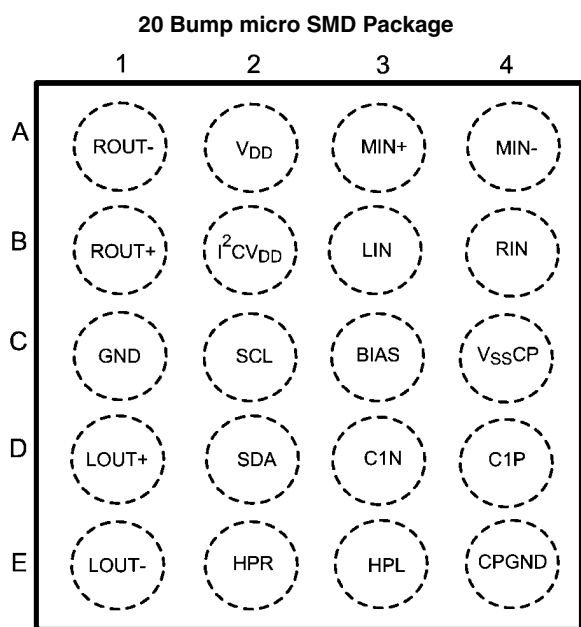
Top View (Bump Side Down) Order Number LM49200TL, LM49200TLX See NS Package Number TLA20BBA
