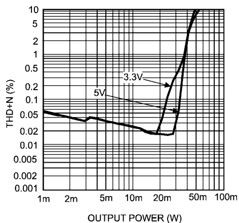
THD+N vs Output Power V_{DD} = 3.3V & 5V , R_L = 32\Omega , f = 1kHz Mode 4, 80kHz BW
