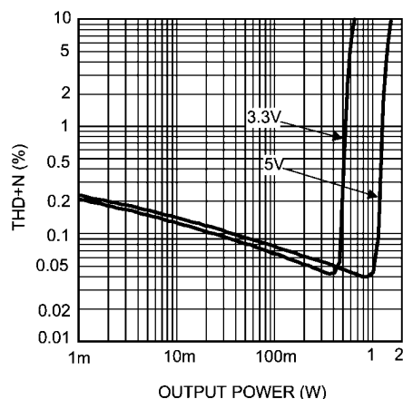
THD+N vs Output Power V_{DD} = 3.3V & 5V , R_L = 8\Omega BTL, f = 1kHz Mode 2, 80kHz BW
