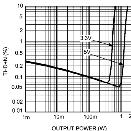
THD+N vs Output Power V_{DD} = 3.3V & 5V , R_L = 8\Omega , f = 1kHz Mode 5, 80kHz BW
