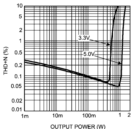
THD+N vs Output Power V_{DD} = 3.3V & 5V , R_L = 8\Omega BTL, f = 1kHz Mode 1, 80kHz BW
