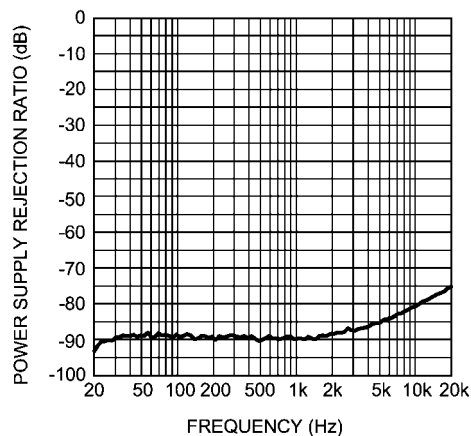
PSRR vs Frequency V_{DD} = 3.3V, V_{RIPPLE} = 200mV_{P-P}, R_L = 32\Omega Mode 4, 80kHz BW
