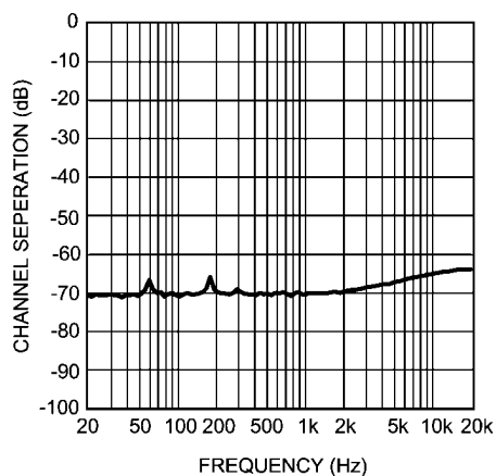
Crosstalk vs Frequency V_{DD} = 3.0V , V_{IN} = 1V_{P-P} , R_L = 32\Omega Mode 8, 80kHz BW
