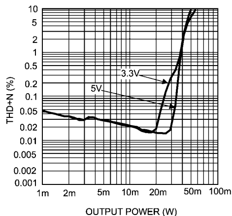
THD+N vs Output Power V_{DD} = 3.3V, V_{RIPPLE} = 200mV_{P-P}, R_L = 32\Omega, f = 1kHz Mode 8, 80kHz BW
