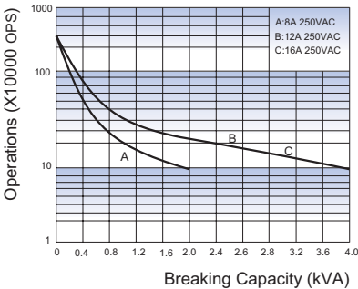
ENDURANCE CURVE
