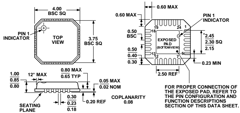
Figure 34. 24-Lead Lead Frame Chip Scale Package [LFCSP_VQ] 4 mm x 4 mm Body, Very Thin Quad (CP-24-2) Dimensions shown in millimeters
