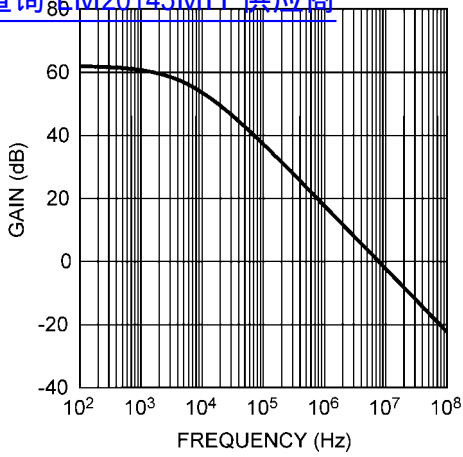
Error Amplifier Gain vs. Frequency 查询"LM20145MH"供应商
