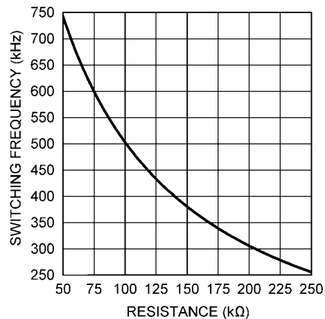
Switching Frequency vs. R T
