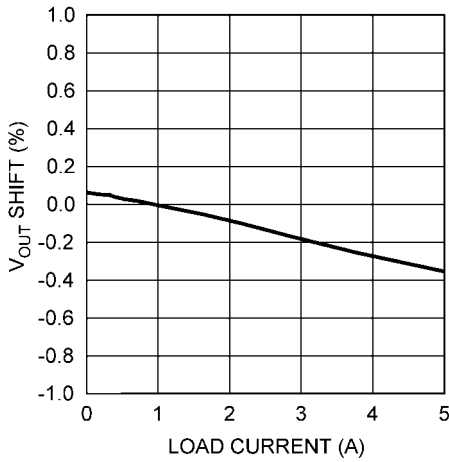
Load Regulation
