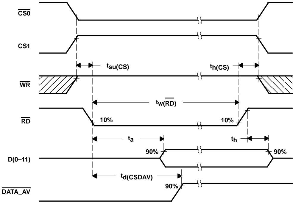
Figure 13. Read Timing Diagram Using \overline{\text{RD}} ( \overline{\text{RD}} -controlled)
