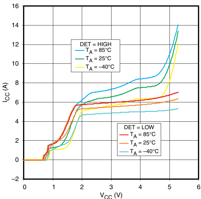
Figure 2. I_{CC} vs V_{CC} , EN = V_{CC}
