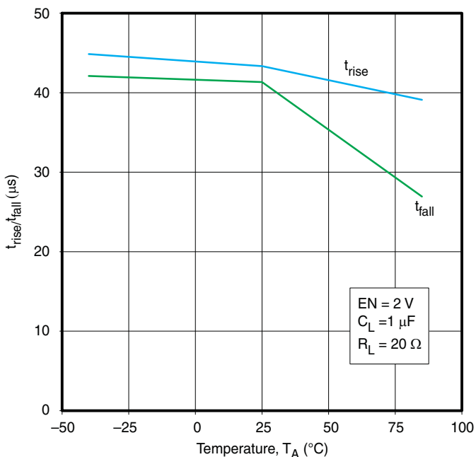
Figure 4. t_{rise}/t_{fall} vs Temperature, V_{CC} = 5.3 V
