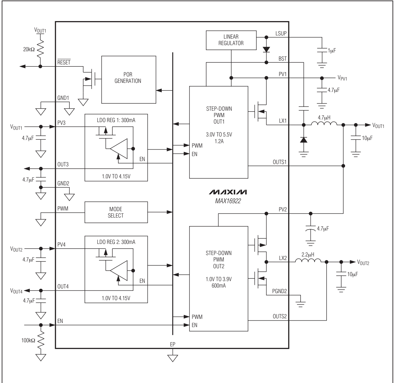
Functional Diagram
