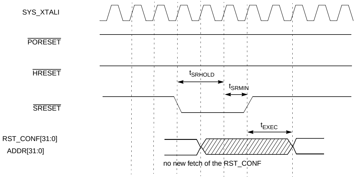
Figure 7. SRESET Behavior
