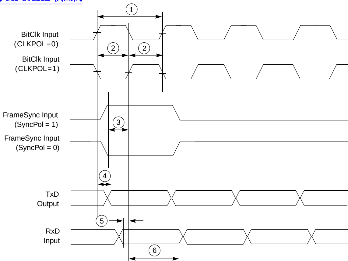
Figure 47. Timing Diagram – 8,16, 24, and 32-bit CODEC/I²S Slave Mode
