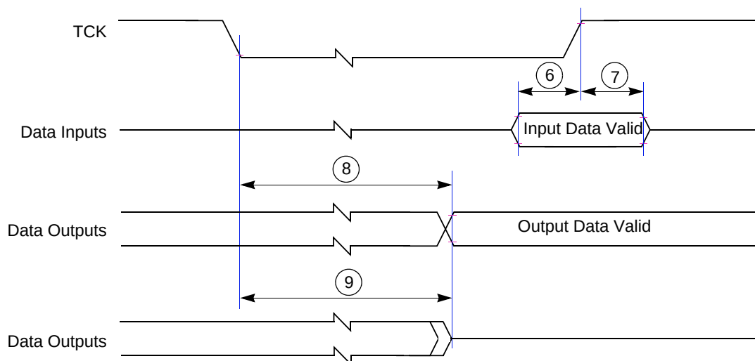
Figure 55. Timing Diagram – JTAG Boundary Scan
