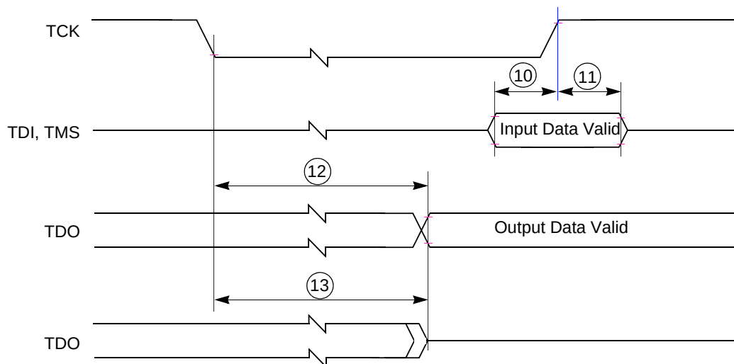
Figure 56. Timing Diagram – Test Access Port
