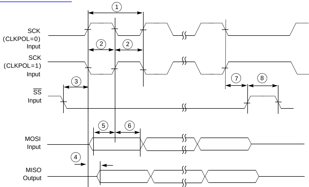
Figure 52. Timing Diagram – SPI Slave Mode, Format 1 (CPHA = 1)
