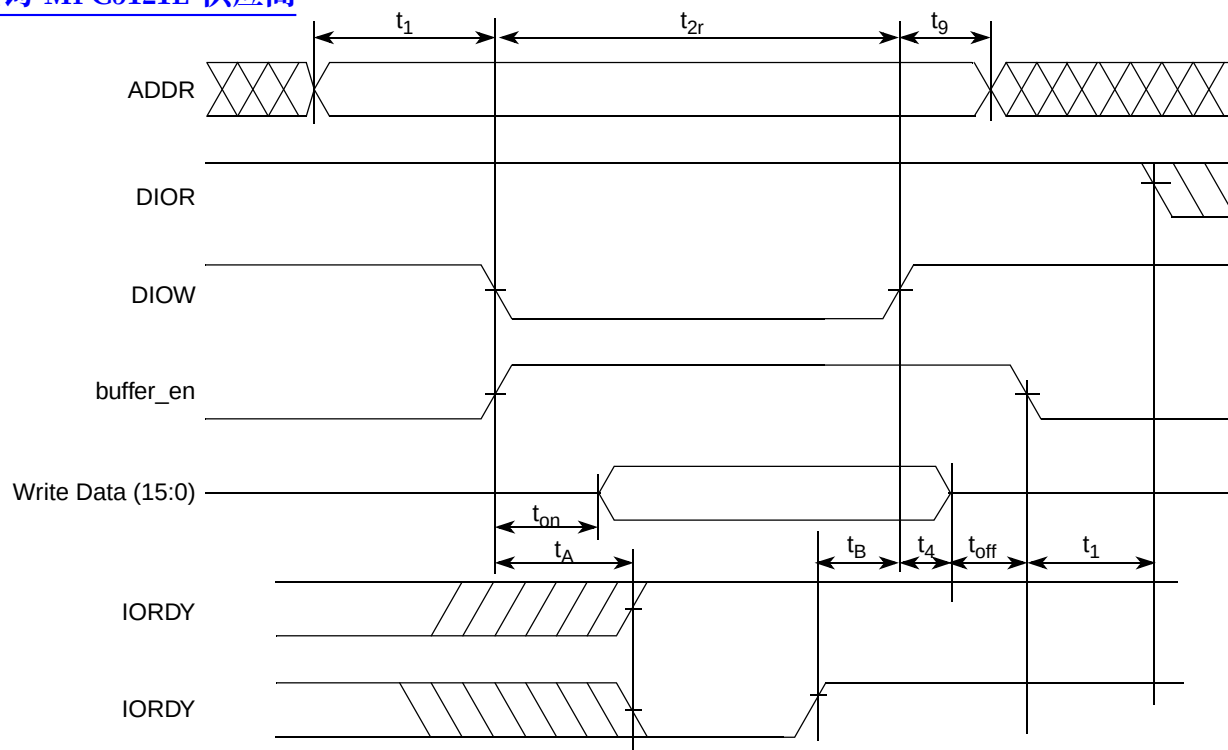
Figure 26. PIO Write Mode Timing
