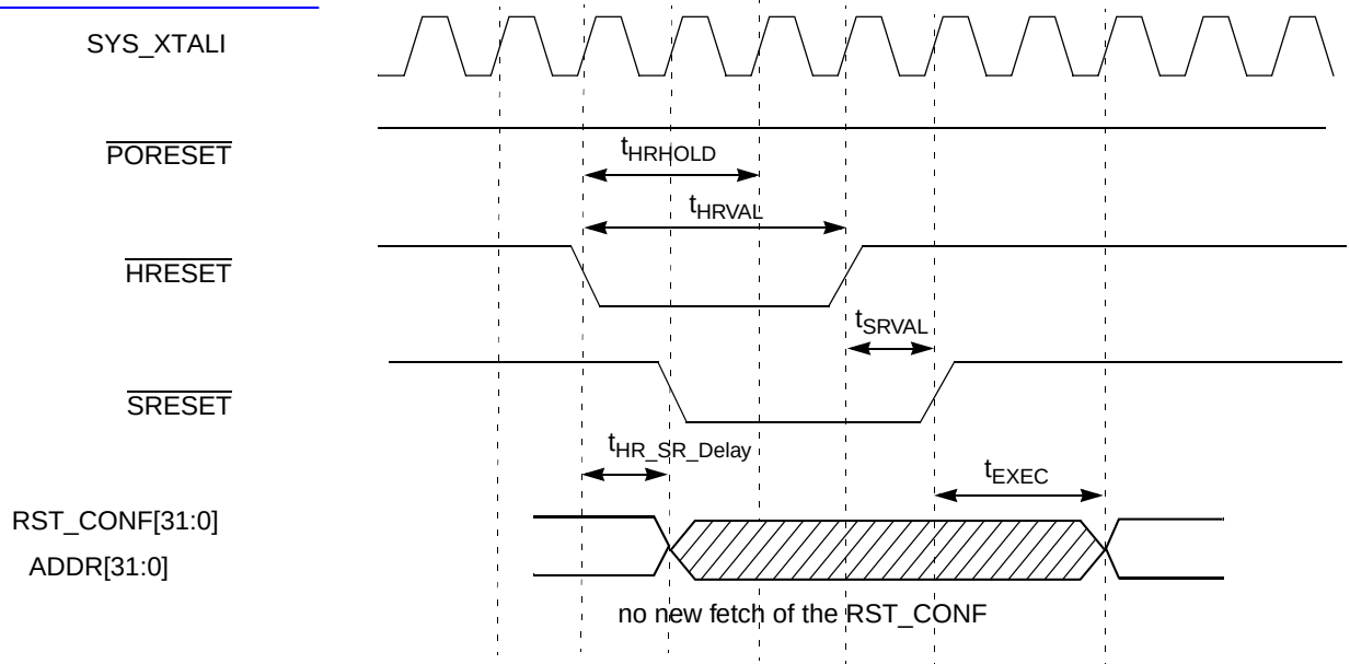
Figure 6. HRESET Behavior
