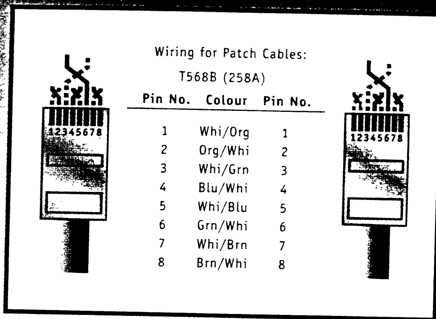
Wiring Diagram
